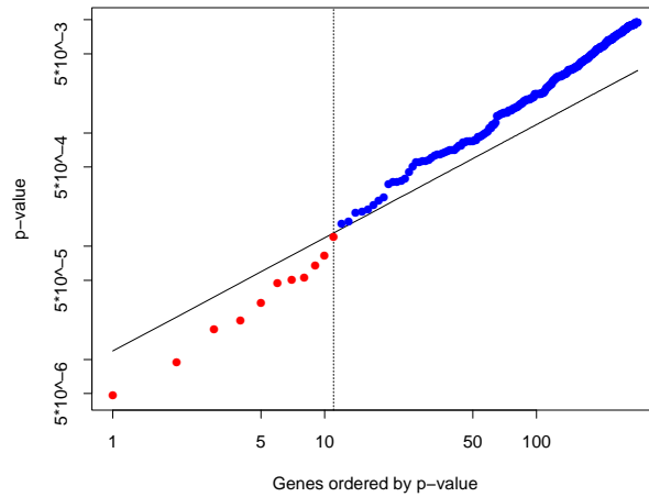
FIGURE 18.19. Microarray example continued. Shown is a plot of the ordered p -values p_{(j)} and the line 0.15 \cdot (j/12, 625) , for the Benjamini–Hochberg method. The largest j for which the p -value p_{(j)} falls below the line, gives the BH threshold. Here this occurs at j = 11 , indicated by the vertical line. Thus the BH method calls significant the 11 genes (in red) with smallest p -values.
